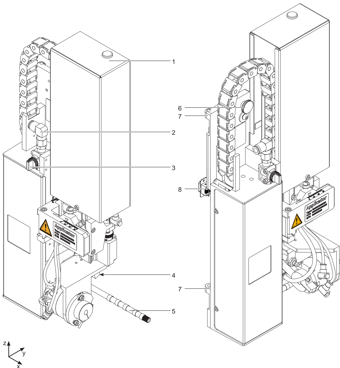
Fig. 2 Device overview
